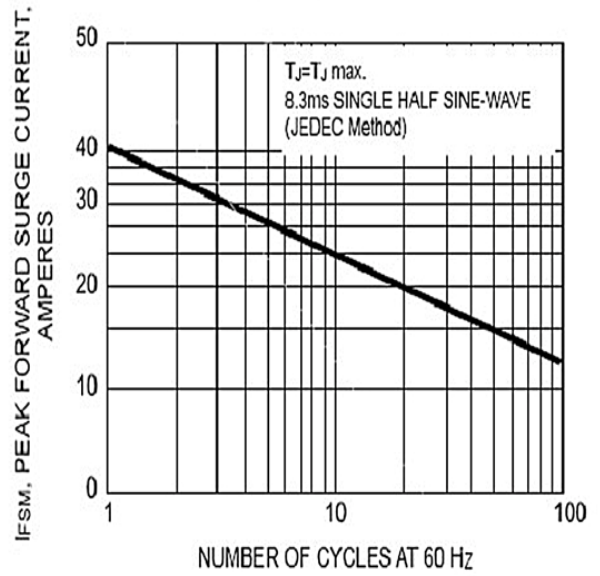
FIG. 6 - MAXIMUM NON-REPETITIVE FORWARD SURGE CURRENT UNIDIRECTIONAL ONLY
