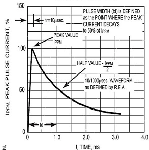
FIG. 3 - PULSE WAVEFORM
