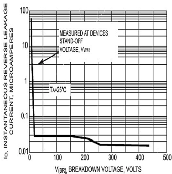
FIG. 7 - TYPICAL REVERSE LEAKAGE CHARACTERISTICS
