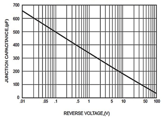
FIG. 4-TYPICAL JUNCTION CAPACITANCE
