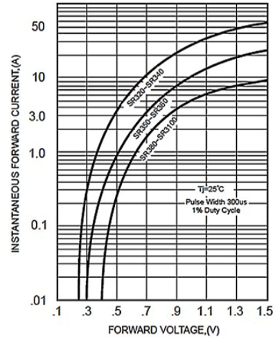
FIG. 2-TYPICAL FORWARD CHARACTERISTICS
