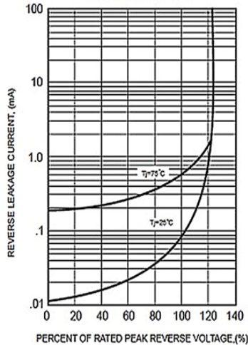
FIG. 5 - TYPICAL REVERSE CHARACTERISTICS
