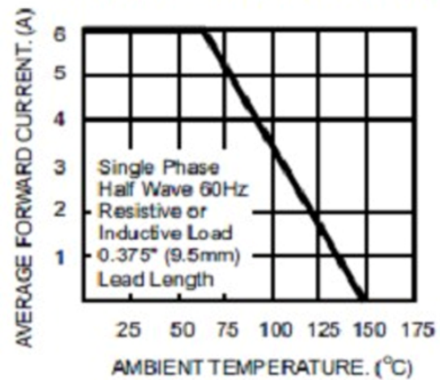
FIG.2- MAXIMUM AVERAGE FORWARD CURRENT DERATING
