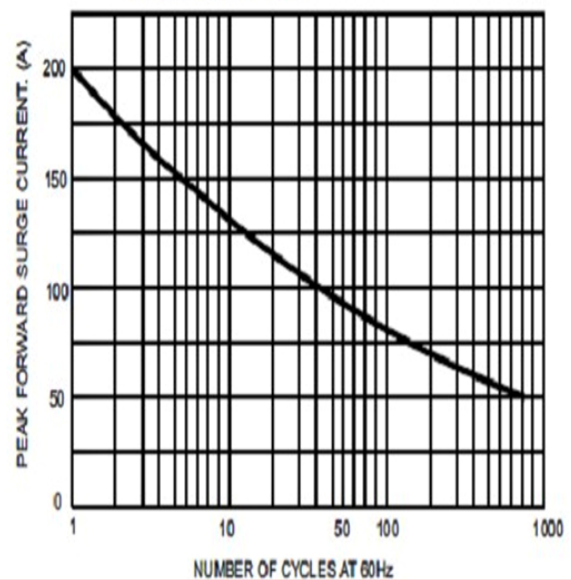
FIG.4- MAXIMUM NON-REPETITIVE FORWARD SURGE CURRENT
