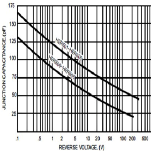
FIG. - TYPICAL JUNCTION CAPACITANCE
