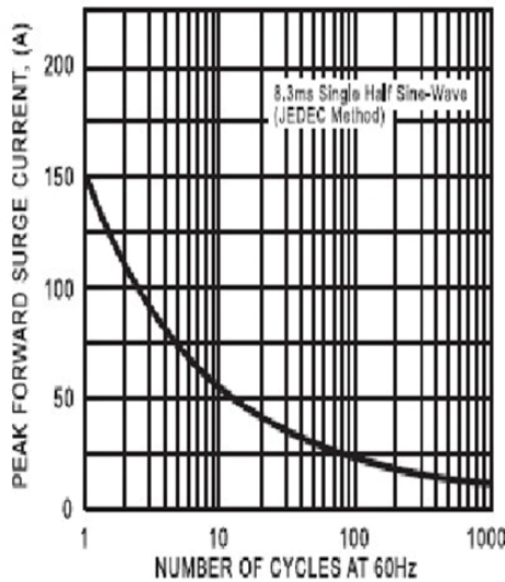
FIG. 1 - MAXIMUM NON-REPETITIVE FORWARD SURGE CURRENT
