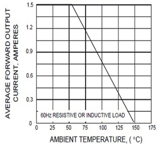
FIG.2 - DERATING CURVE FOR OUTPUT RECTIFIED CURRENT
