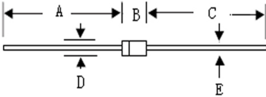
DO-41
