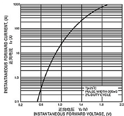
FIG. 4 - 正向特性曲线(典型) FIG. 4 - TYPICAL FORWARD CHARACTERISTICS
